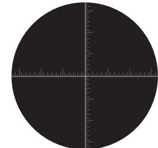
6 Object Plate From the center point, there are gradation of 0.5mm on 10mm of vertical and horizontal lines so that the object size can be easily identified.
